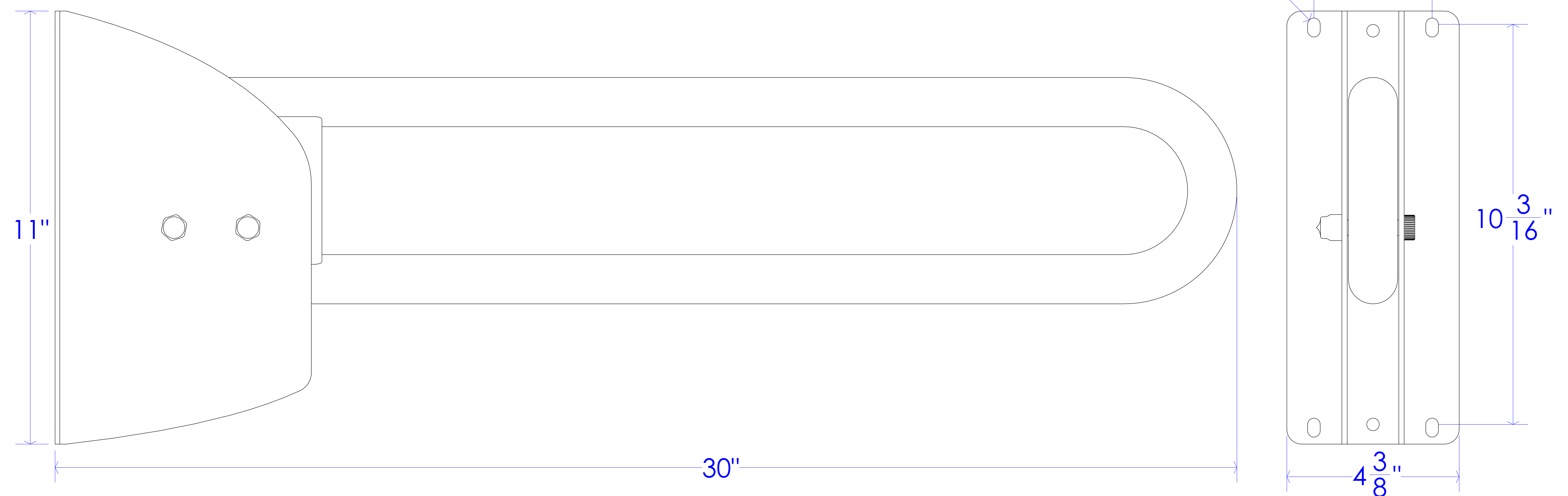
Front View (grab bar in down position)
