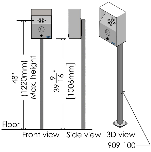
Code 909-100 Heavy Duty Pedestal
