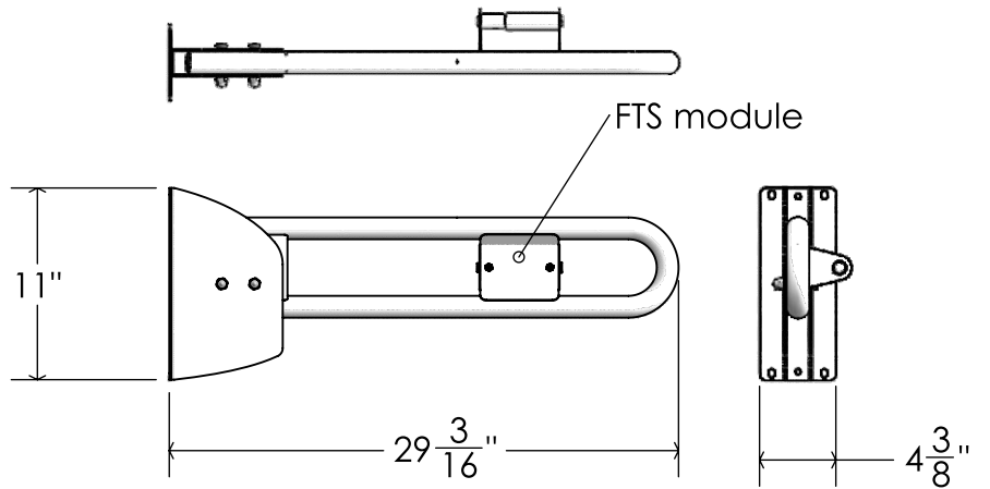
Front View (grab bar in down position)
