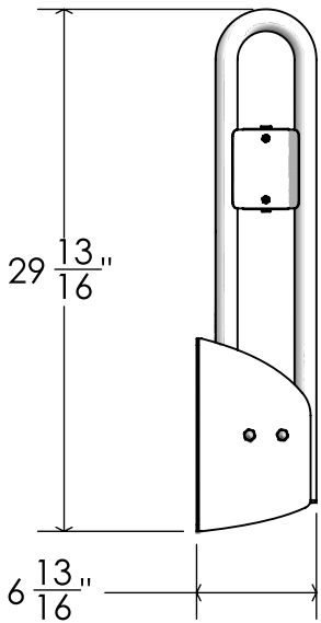
Front View (grab bar in up position)
